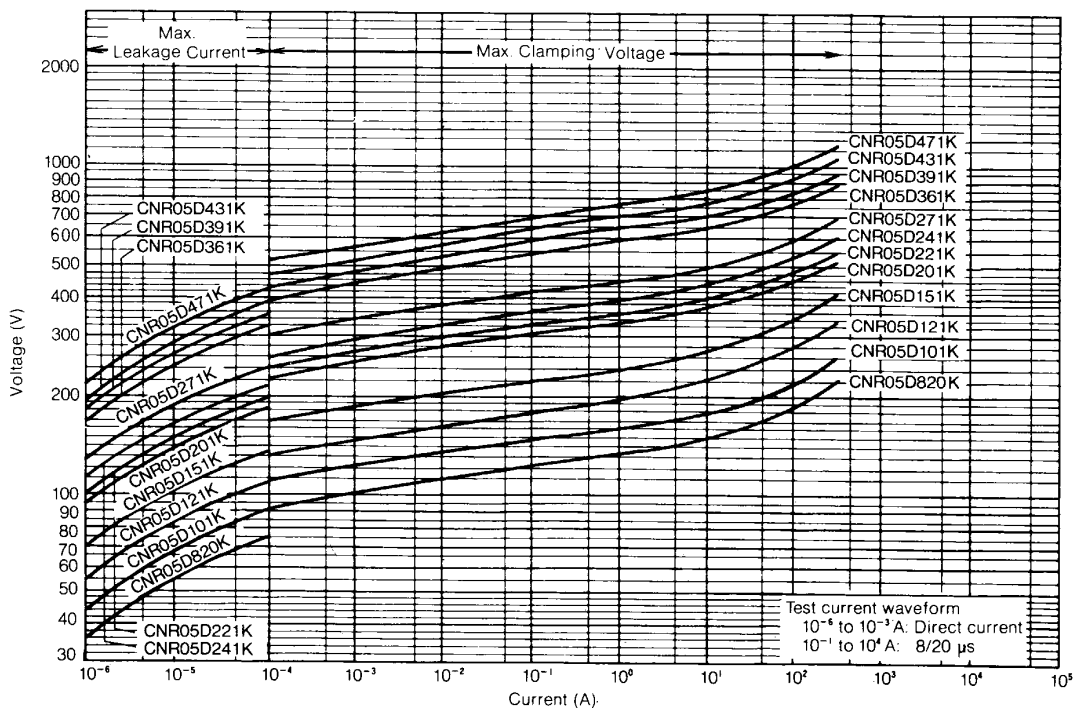
V-I Curve (CNR05D820K to CNR05D471K)
