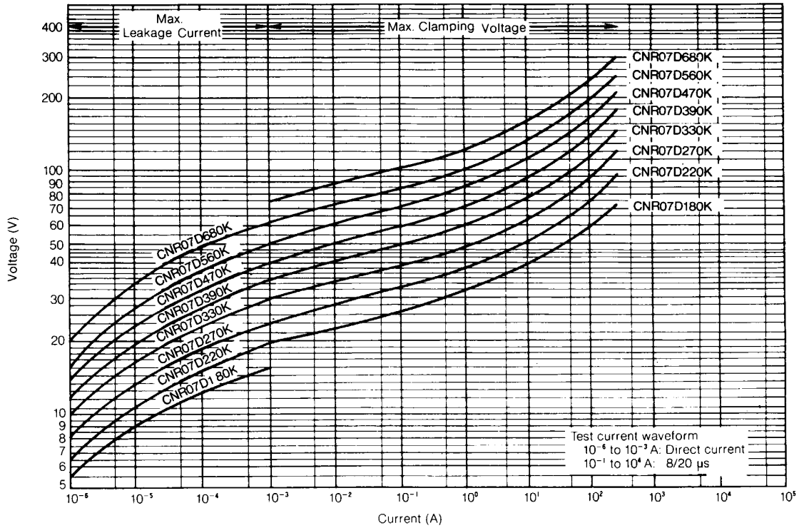
V-I Curve (CNR07D180K to CNR07D680K)
