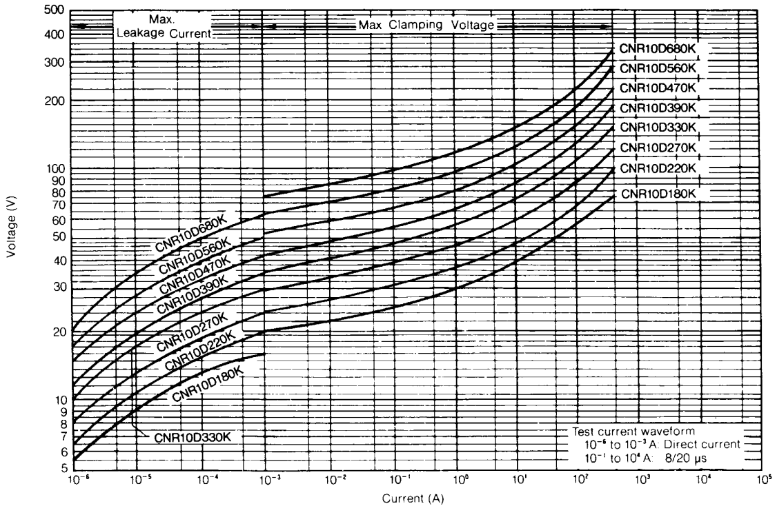
V-I Curve (CNR10D180K to CNR10D680K)
