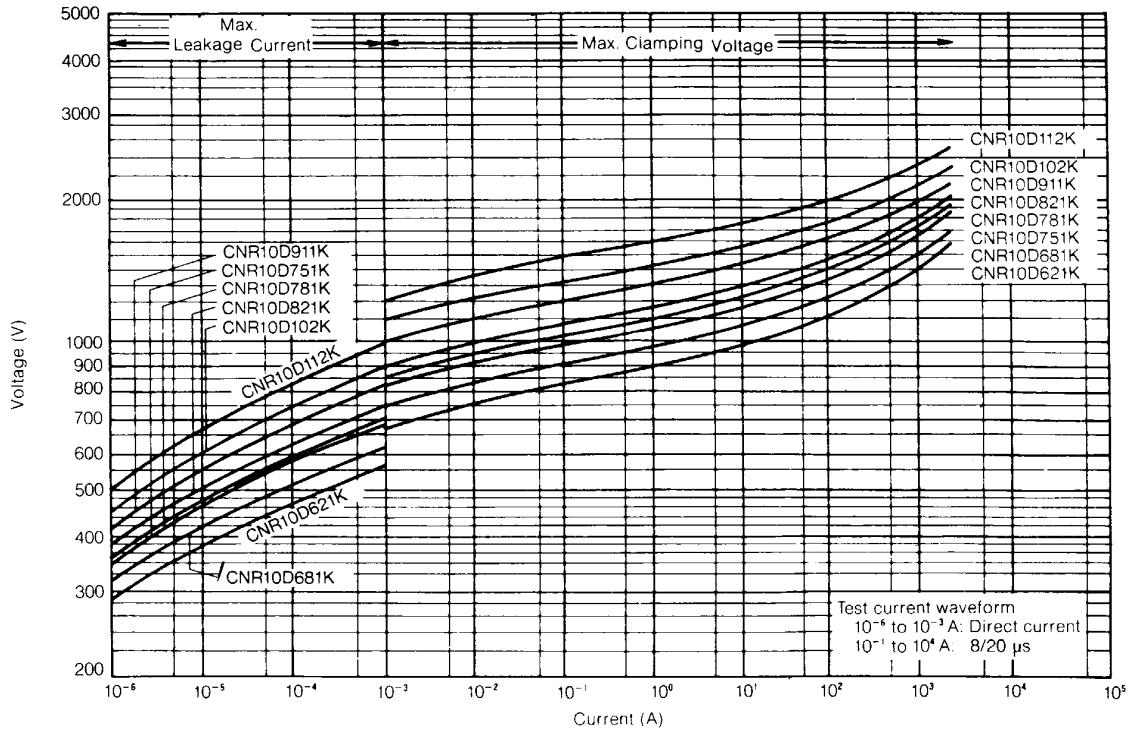
V-I Curve (CNR10D621K to CNR10D112K)
