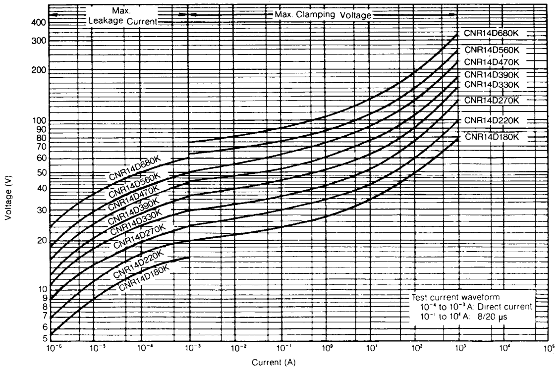
V-I Curve (CNR14D180K to CNR14D680K)
