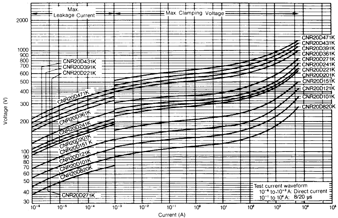
V-I Curve (CNR20D820K to CNR20D471K)
