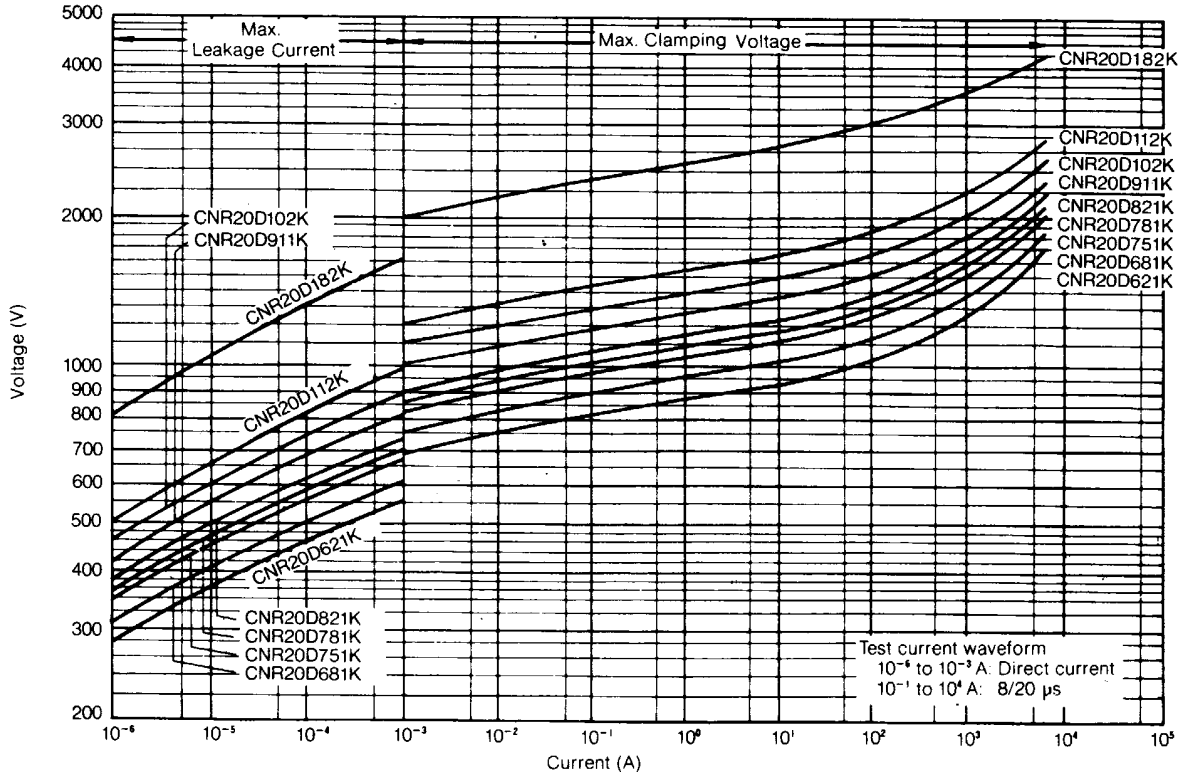
V-I Curve (CNR20D621K to CNR20D182K)
